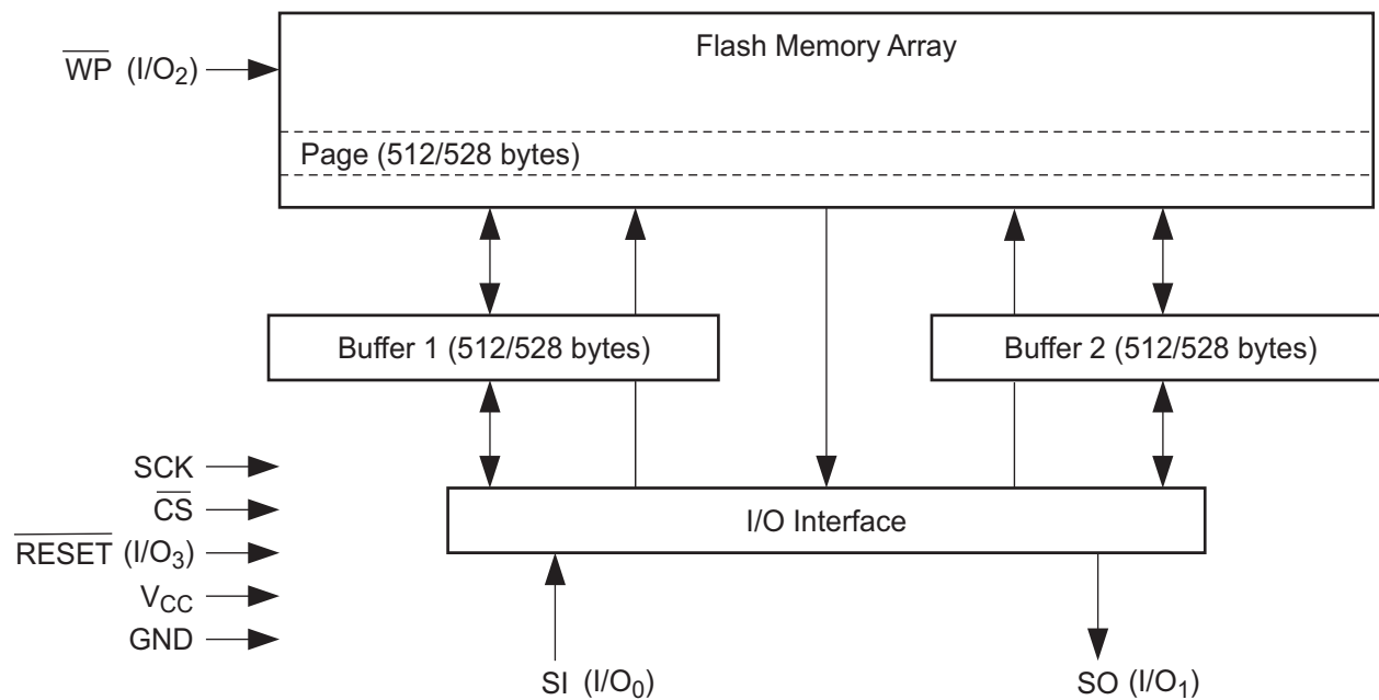
Figure 2-1. Block Diagram
