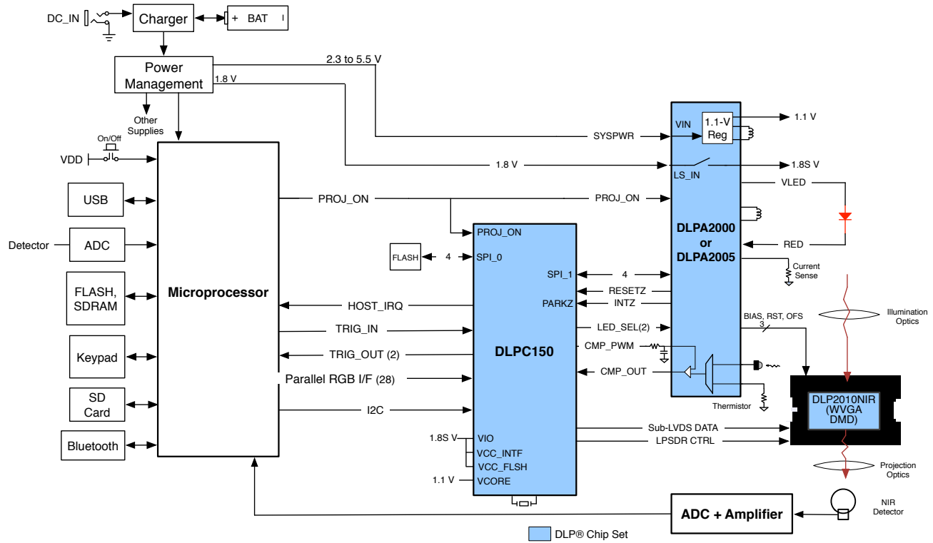
Figure 20. Typical Application Diagram
