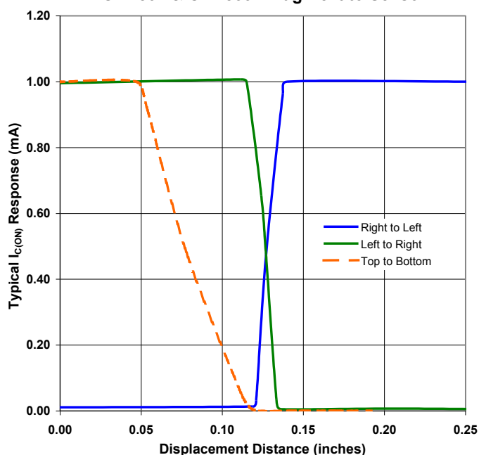
OPB852 & OPB853 - Flag Next to Sensor
