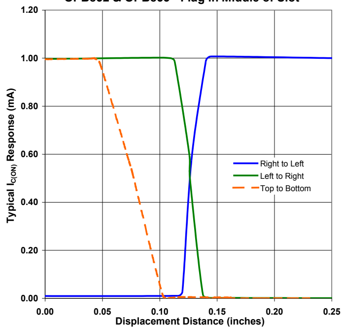
OPB852 & OPB853 - Flag in Middle of Slot
