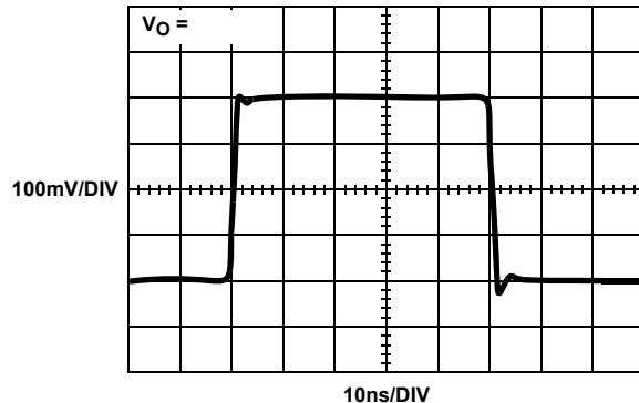
FIGURE 16. SMALL SIGNAL RESPONSE
