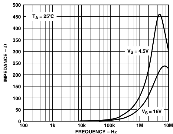
TPC 14. Close-Loop Output Impedance vs. Frequency
