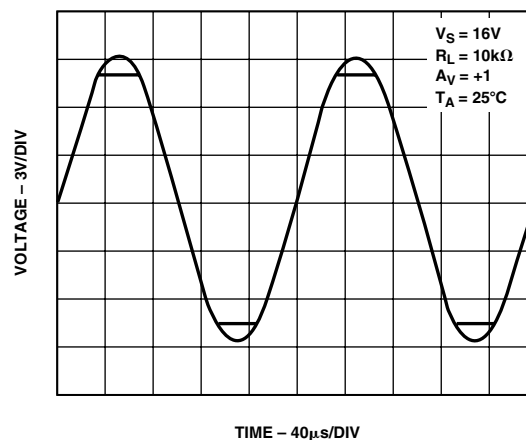
TPC 17. No Phase Reversal
