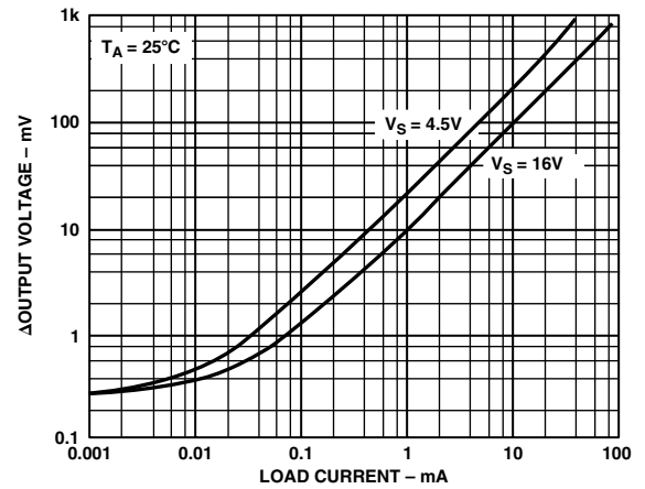
TPC 11. Output Voltage to Supply Rail vs. Load Current
