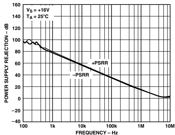
TPC 16. Power Supply Rejection Ratio vs. Frequency
