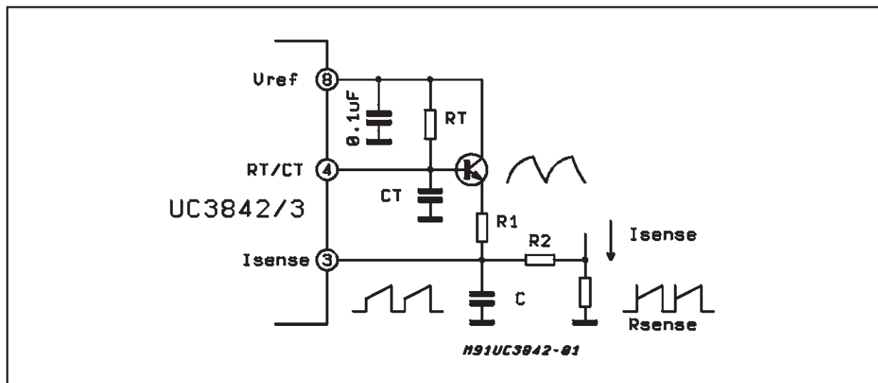
Figure 12 : Slope Compensation.
