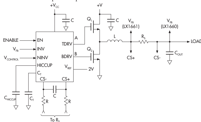
Figure 2 — LX1660 / 1661 General Circuit Configuration
