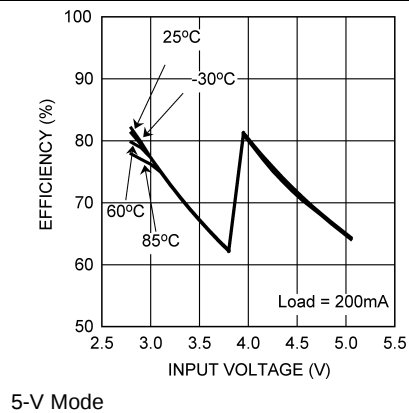
Figure 22. Efficiency vs. Input Voltage
