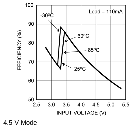
Figure 23. Efficiency vs. Input Voltage
