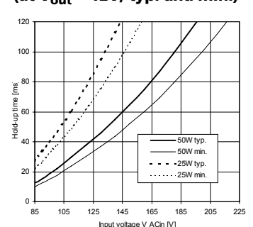
Hold-up time with ACin (at V_{out} = 12\text{V} , typ. and min.)
