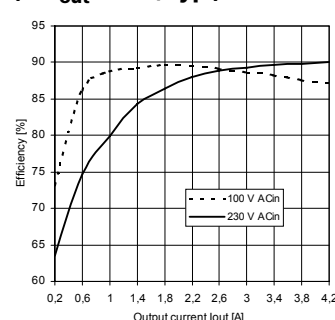
Efficiency (@ V_{out} = 12\text{V} , typ.)
