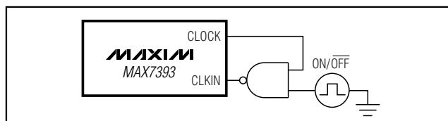
Figure 1. Test Circuit to Enable or Disable the MAX7393 Oscillator
