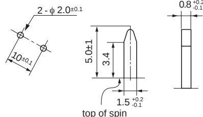
PC board hole dimensions
