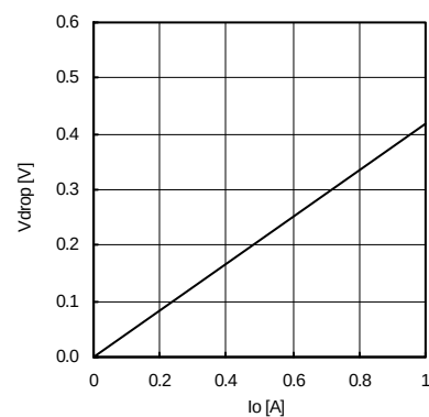
Fig.33 Minimum dropout Voltage2 (VCC=2.4V)
