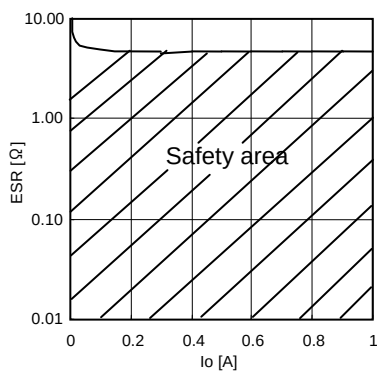
Fig.29 ESR-IO characteristics (Co=2.2μF)
