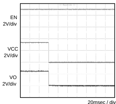
Fig.4 OFF sequence 1 \text{Co}=2.2\mu\text{F}
