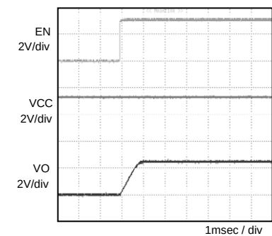
Fig.5 Input sequence2 \text{Co}=2.2\mu\text{F}
