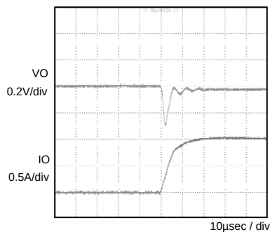
Fig.1 Transient Response(0→1.0A) \text{Co}=2.2\mu\text{F}
