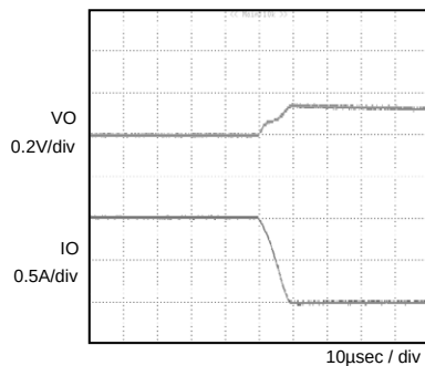
Fig.2 Transient Response(1.0→0A) \text{Co}=2.2\mu\text{F}
