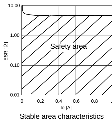
Stable area characteristics
