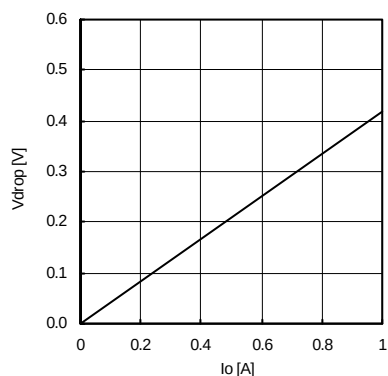
Fig.34 Minimum dropout Voltage3 (VCC=3.3V)
