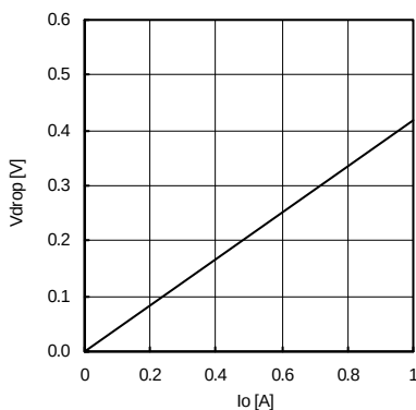
Fig.35 Minimum dropout Voltage4 (VCC=5.0V)
