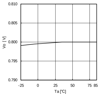
Fig.7 Ta-VFB
