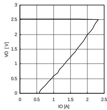
Fig.21 OCP (VCC=5V, VO=2.5V)
