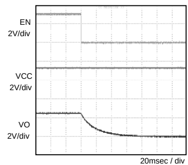
Fig.6 OFF sequence 2 \text{Co}=2.2\mu\text{F}
