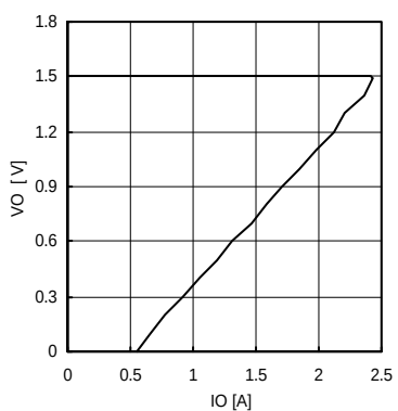
Fig.23 OCP (VCC=5V, VO=1.5V)
