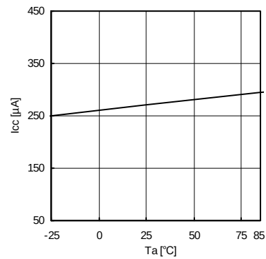
Fig.9 Ta-ICC
