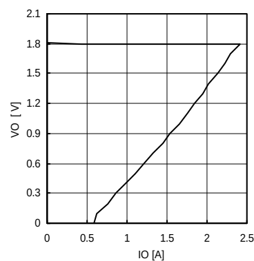
Fig.22 OCP (VCC=5V, VO=1.8V)
