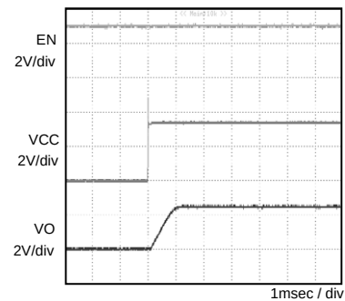
Fig.3 Input sequence1 \text{Co}=2.2\mu\text{F}
