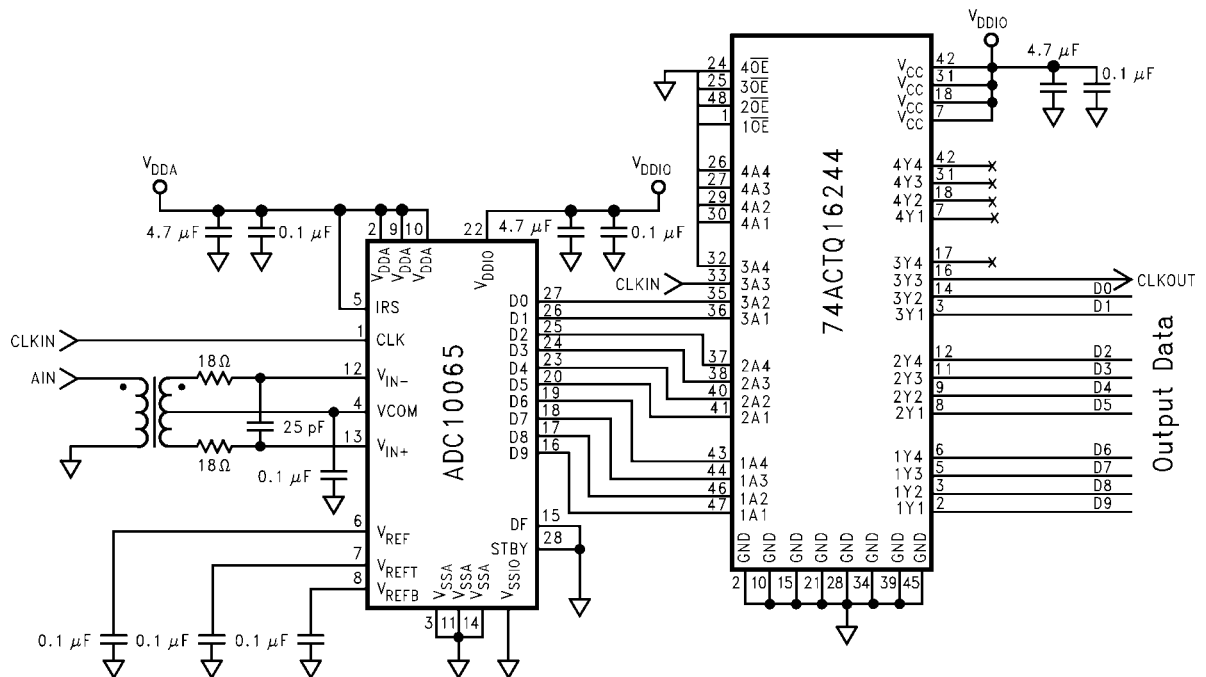
FIGURE 5. A Simple Application Using a Differential Driving Source
