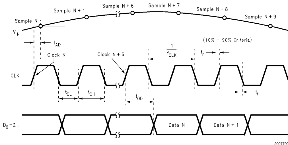
FIGURE 1. Clock and Data Timing Diagram
