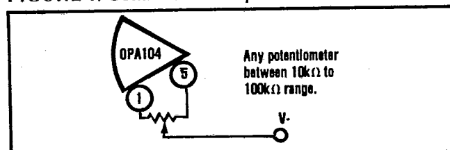
FIGURE 2. External Nulling of Offset Voltage.
