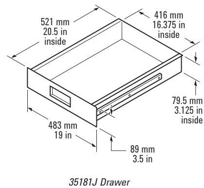
35181J Drawer
