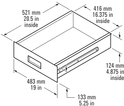
35181M Drawer
