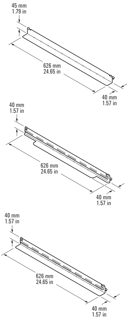
3rd party rail kit (E3664AC)
