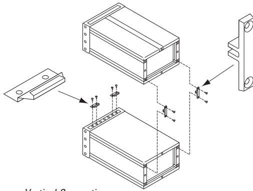
Vertical Connection
