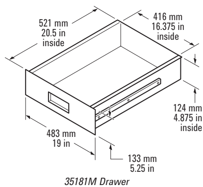
35181M Drawer
