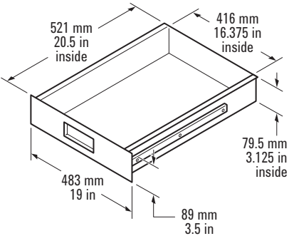
35181J Drawer
