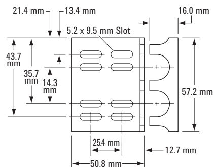
Standard slide bracket dimensions
