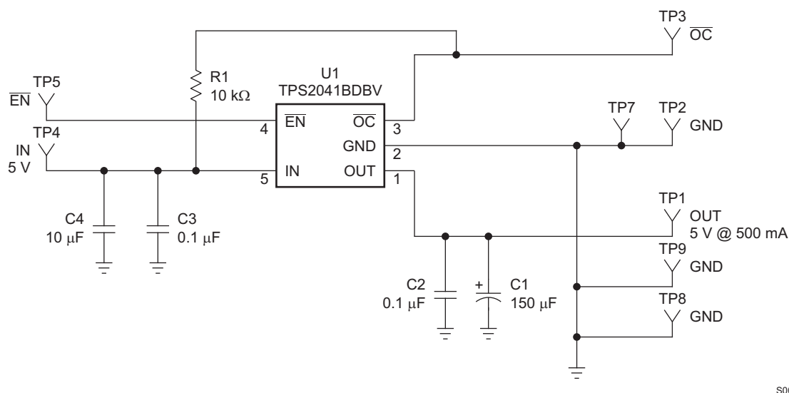
Figure 8. TPS2041B EVM Schematic
