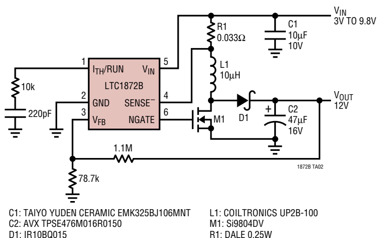
LTC1872B 12V/500mA Boost Converter
