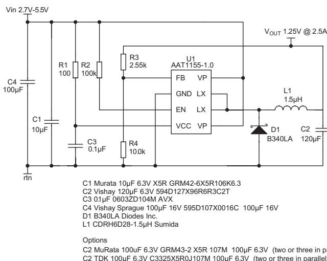
Figure 3. AAT1155 Evaluation Board with adjustable output
