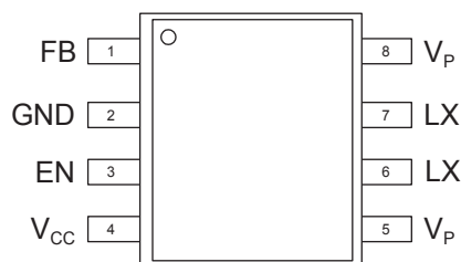
MSOP-8
