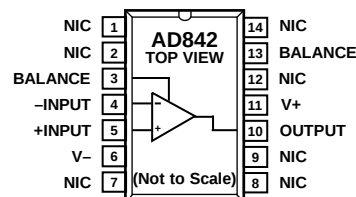
Figure 1. PDIP (N-14) and CERDIP (Q-14)
