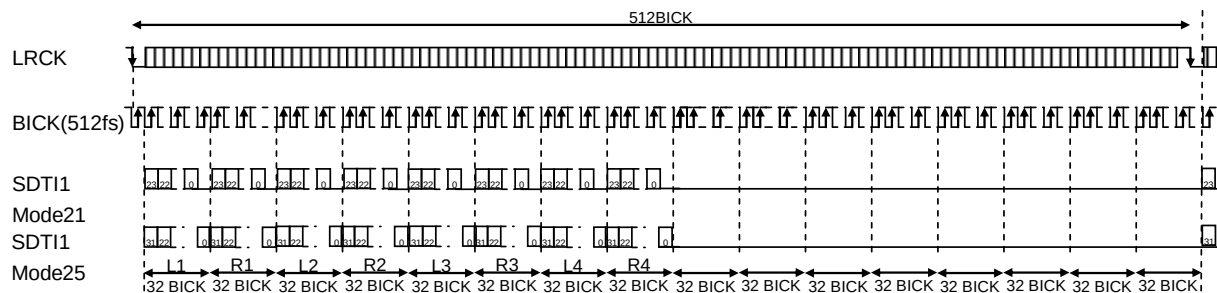
Figure 24. Mode 21/25 Timing
