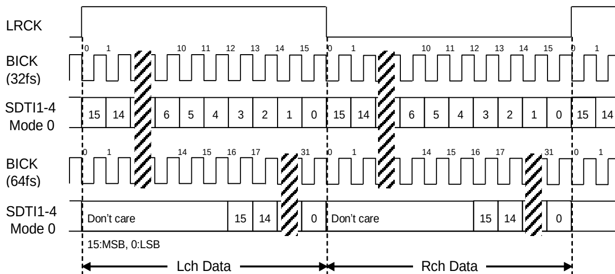
Figure 11. Mode 0 Timing
