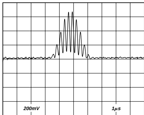
Figure 8. Zoom on Modulated Pulse, NTSC
