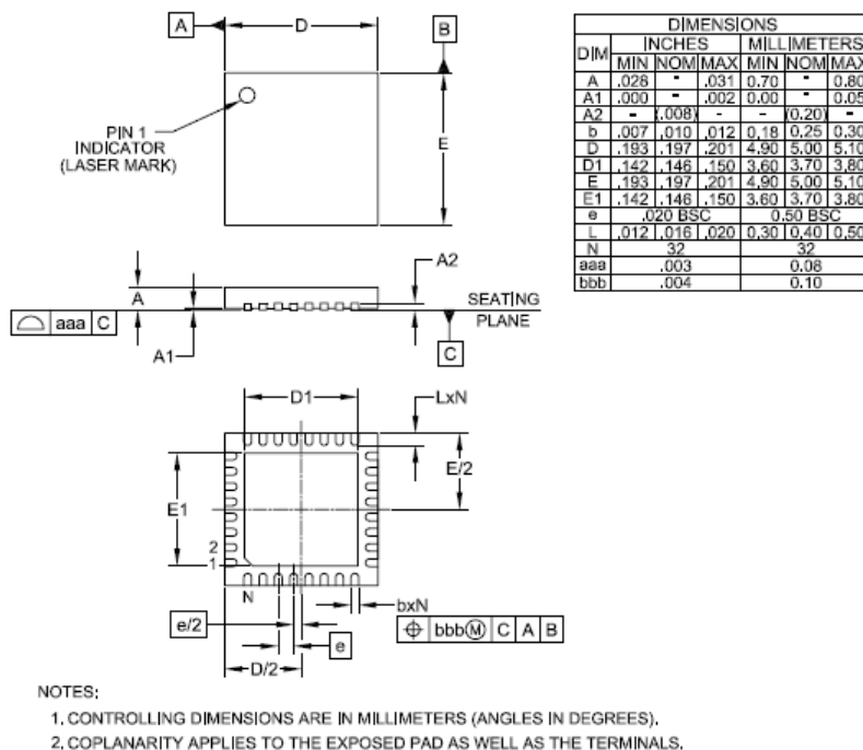
Figure 58 Package Outline Drawing
