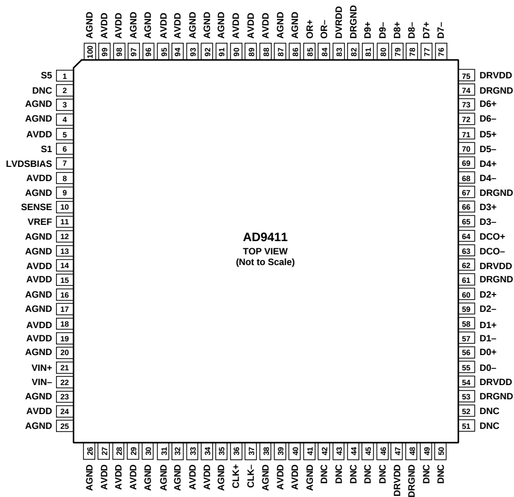
Figure 3. TQFP/EP Pinout
