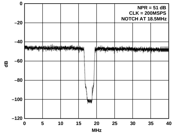
Figure 36. Noise Power Ratio Plot (200 MSPS Grade)
