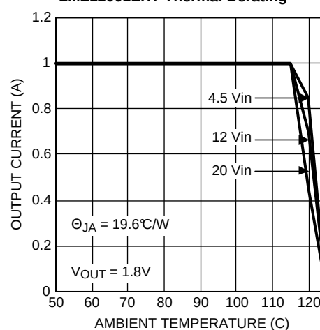
LMZ12001EXT Thermal Derating
