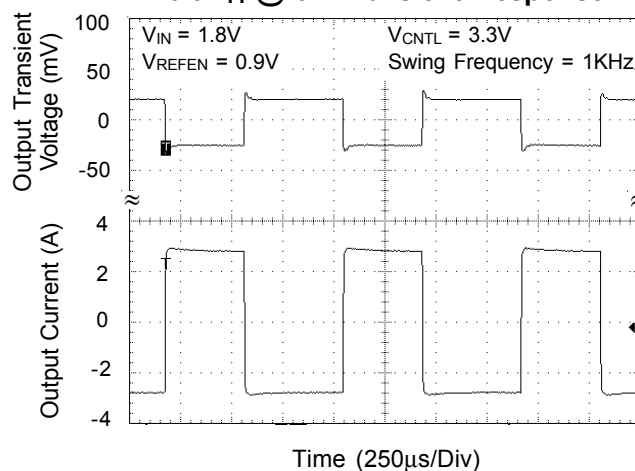
0.9V TT @ 3A Transient Response
