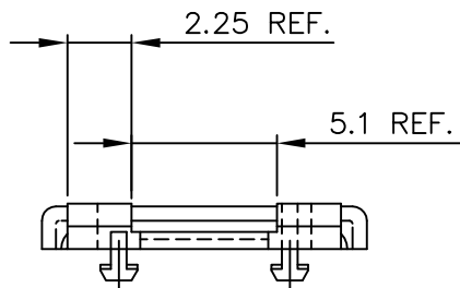
-103LF MIDDLE MALE KEY
