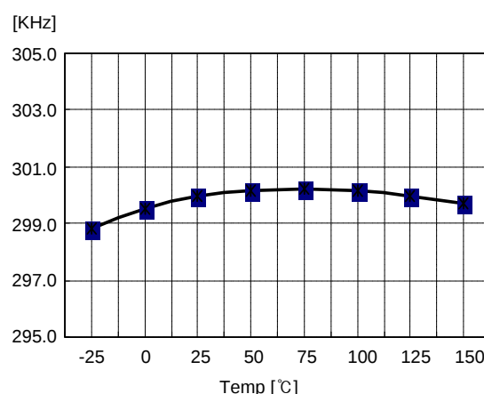
Figure 8. Operating Frequency vs. Temp
