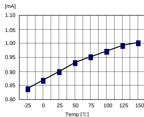
Figure 9. Feedback Source Current vs. Temp
