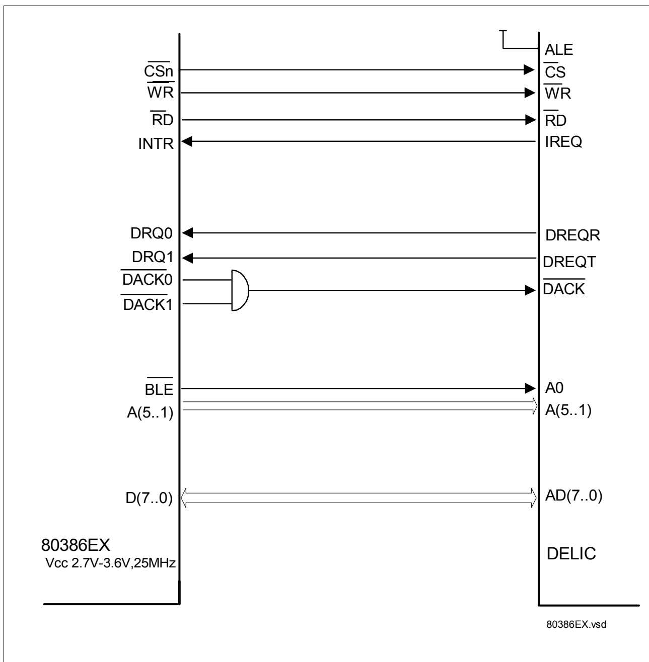
Figure 92 DELIC Connection to Intel 80386EX (Demuxed Configuration)
