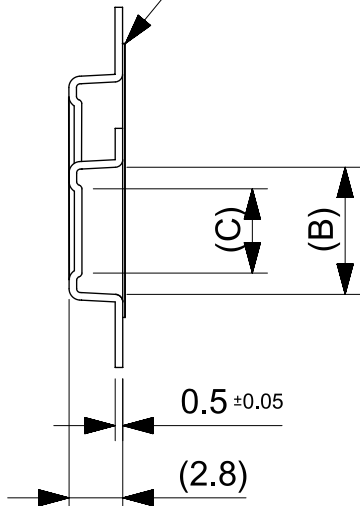
SECT. X-X
