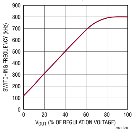
LT3971-X Frequency Foldback
