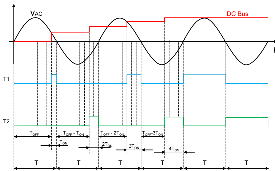
Figure 17. Digital Inrush Current Limiter function: sequence of driving the SCR
