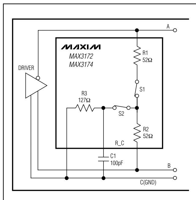
Figure 10. V.35 Driver
