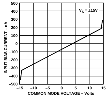
Figure 8. Input Bias Current vs. Common-Mode Voltage
