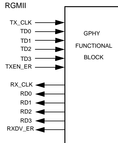
Figure 5. RGMII Signals
