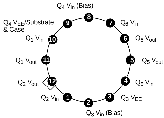
Pin Connection Diagram (Top View)
