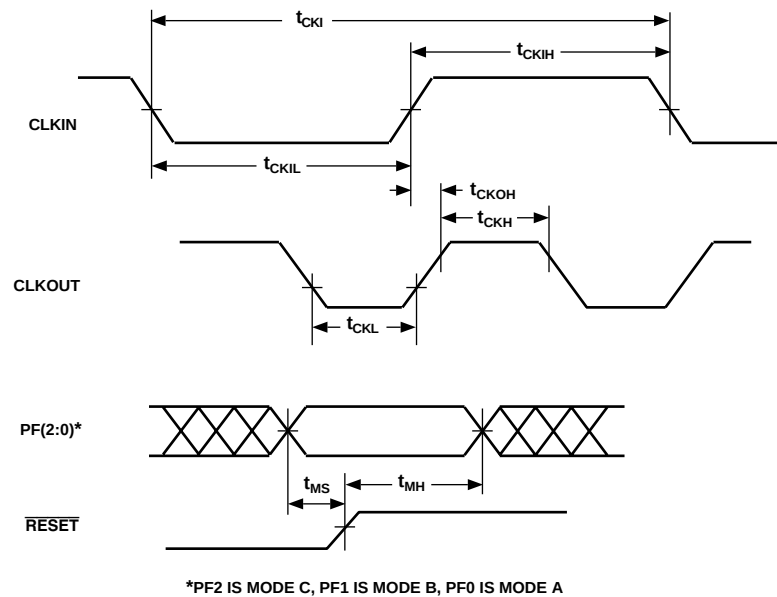
Figure 8. Clock Signals
