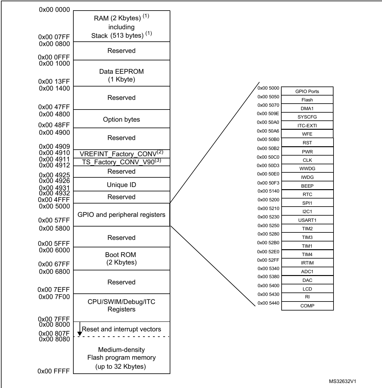
Figure 9. Memory map
