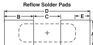
FIGURE 4 - RECOMMENDED MOUNTING PAD GEOMETRIES in inches (millimeters)
