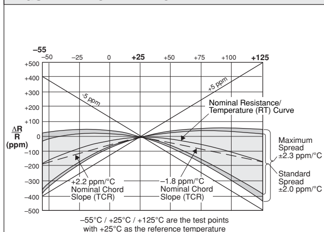
FIGURE 1 - NOMINAL TCR
