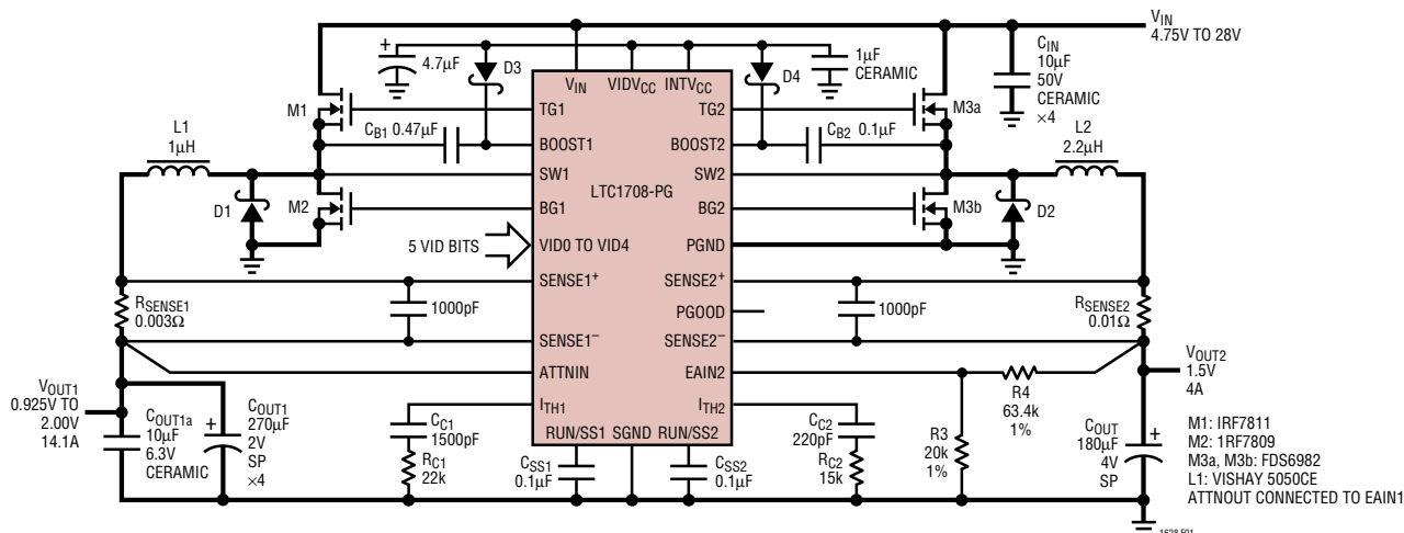
Figure 1. High Efficiency VID Controlled, 2-Output Step-Down Converter
