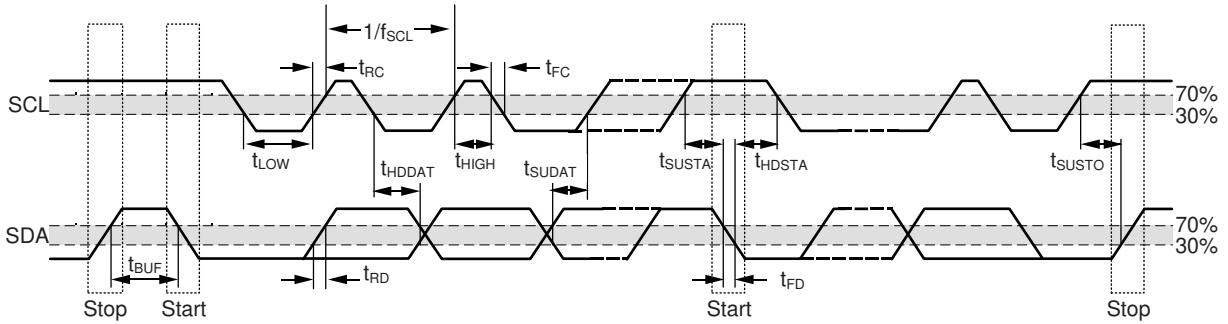
Figure 5-1. I²C Detailed Timing Diagram
