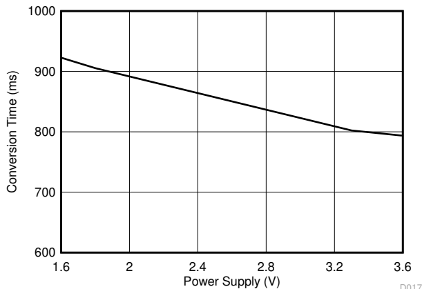
Figure 5-9. Conversion Time vs Power Supply
