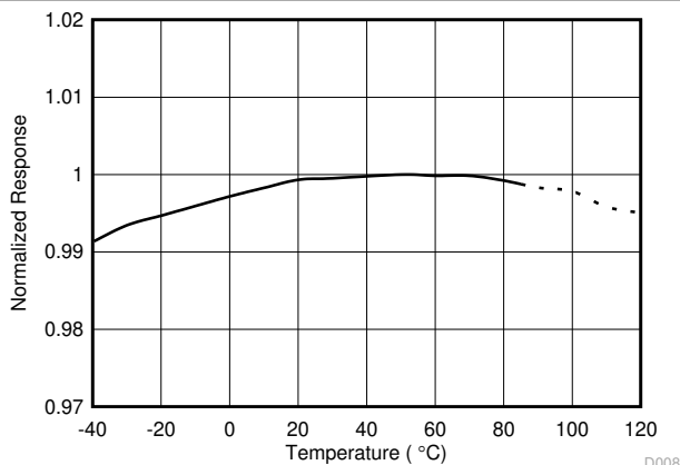
Figure 5-13. Normalized Response vs Temperature (Grade 3)
