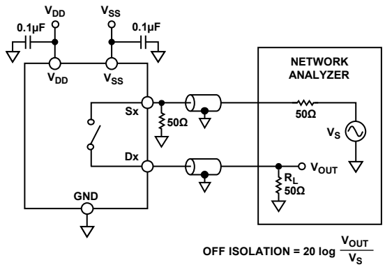
Figure 31. Off Isolation
