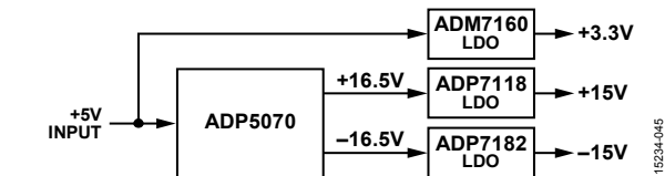
Figure 47. Bipolar Power Solution
