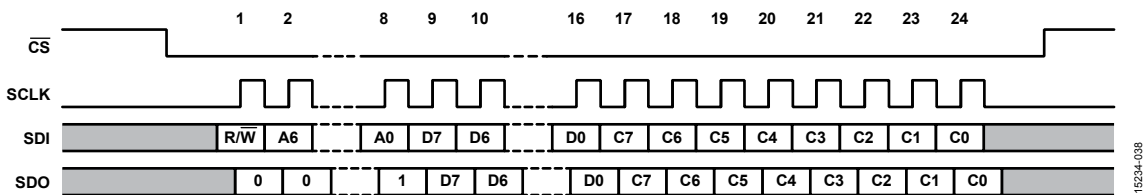
Figure 44. Example of an SPI Frame When Four ADGS5412 Devices Are Connected in Daisy-Chain Mode
