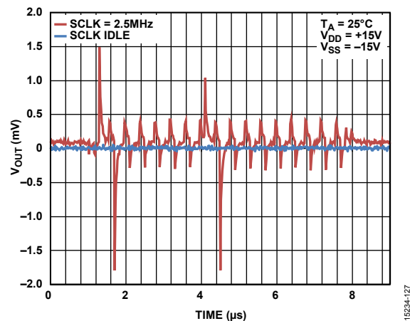
Figure 27. Digital Feedthrough
