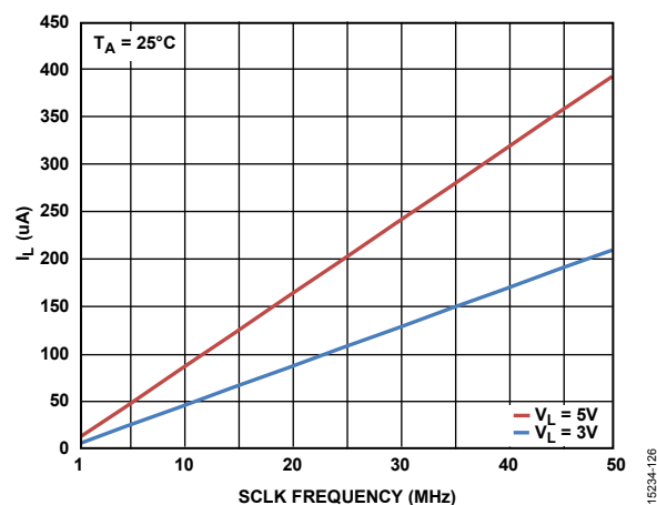
Figure 26. I_L vs. SCLK Frequency When \overline{CS} Is High
