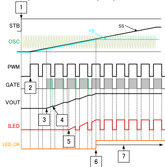
Figure 24. Startup waveform
