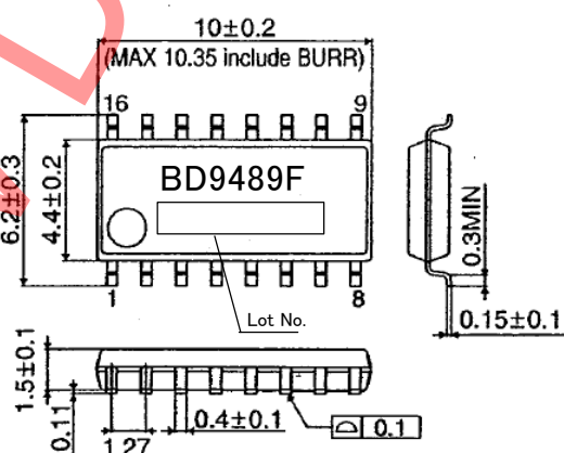
Figure 4. Physical Dimension Tape and Marking Diagram
