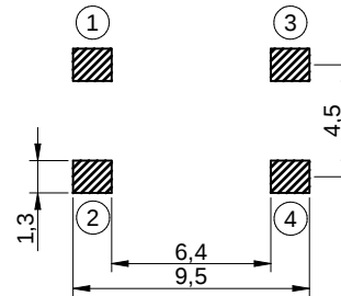
P.C.B. MOUNTING PLAN
