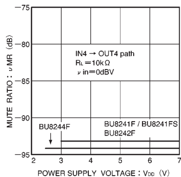
Fig. 14 Mute ratio vs. power supply voltage
