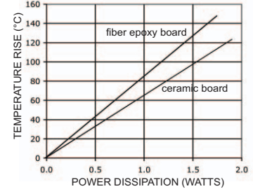
POWER DERATING
