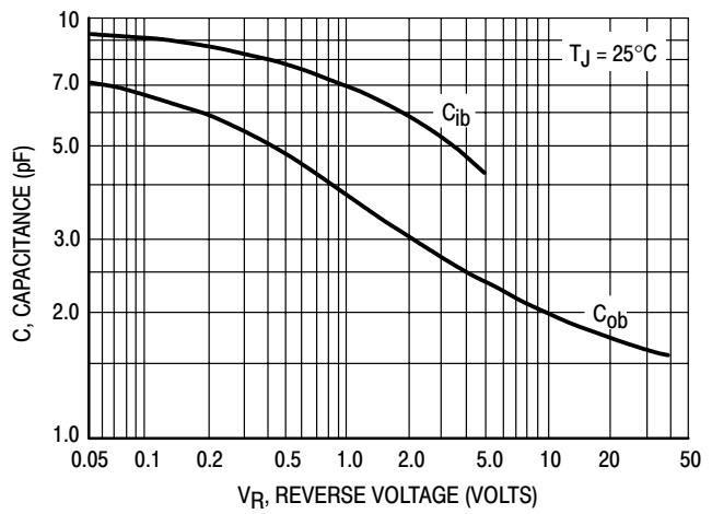
Figure 13. Capacitance
