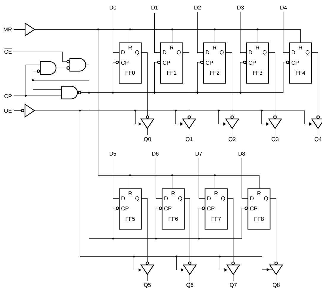
Fig 3. Logic diagram
