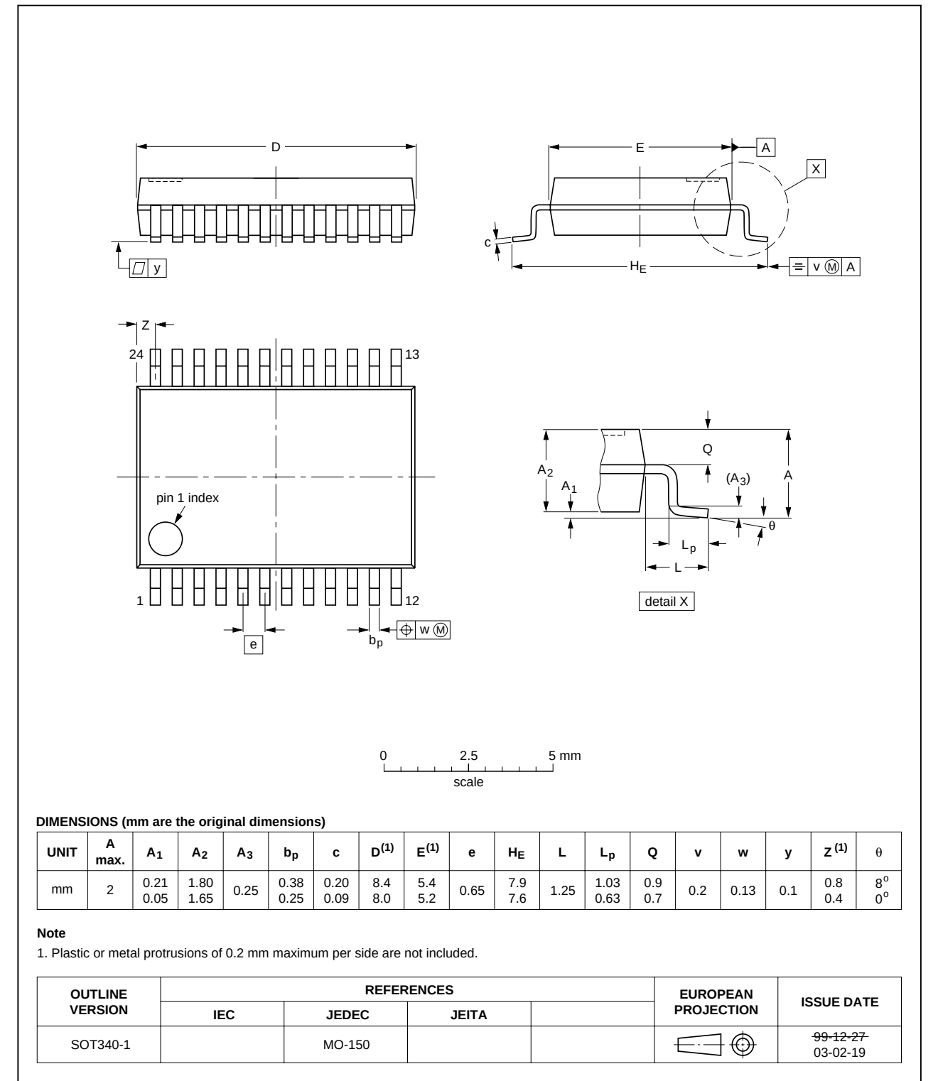
Fig 12. Package outline SOT340-1 (SSOP24)
