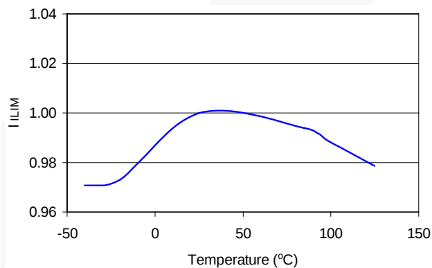
Figure 9. I_{LIM} Current ( I_{ILIM} ) vs. Temperature, Normalized
