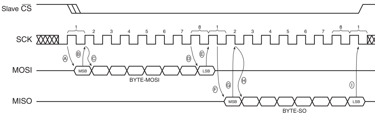
Figure 17-5. Atmel RapidS Mode
