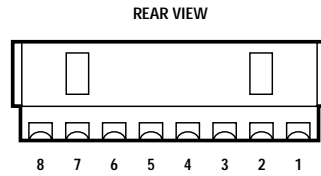
Figure 2. Pinout.
